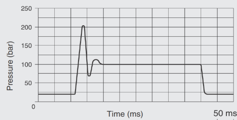
Response times and peak pressure PVV101-1-20 / -25
