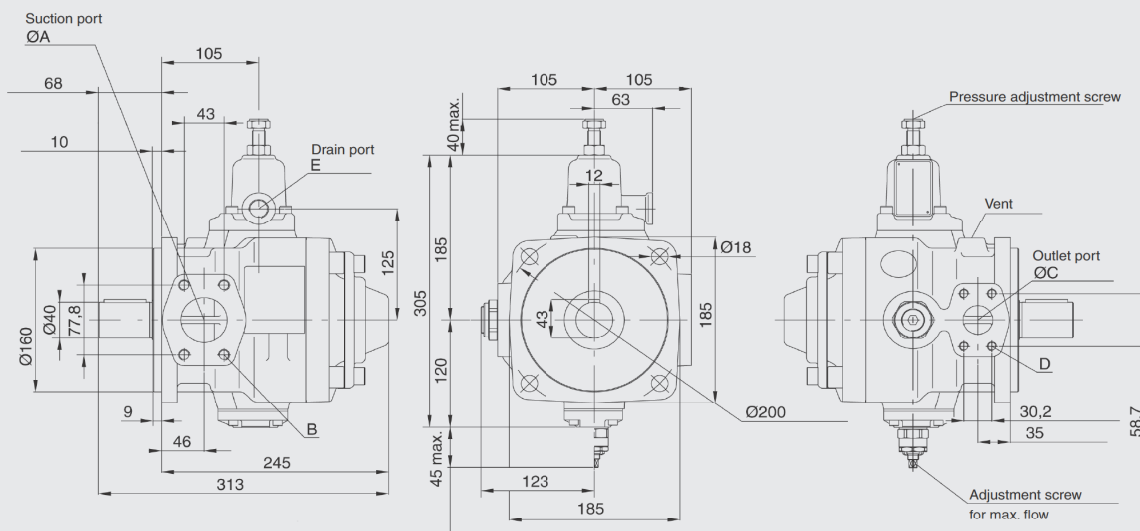
PVV101-3-63 / -80 / -100 (F / F UNC)
