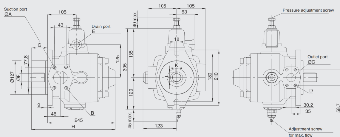
PVV101-3-63 / -80 / -100 (FS / US)
