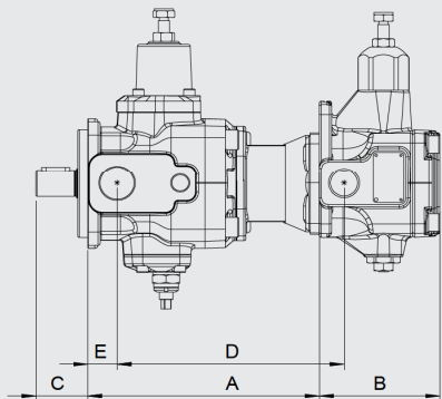
Multiple pumps Front pump PVV101-1- ... F
