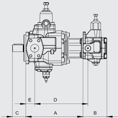
Multiple pumps Front pump PVV101-3- ... F
