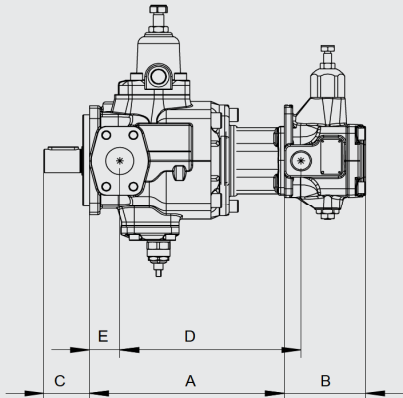
Multiple pumps Front pump PVV101-2- ... F
