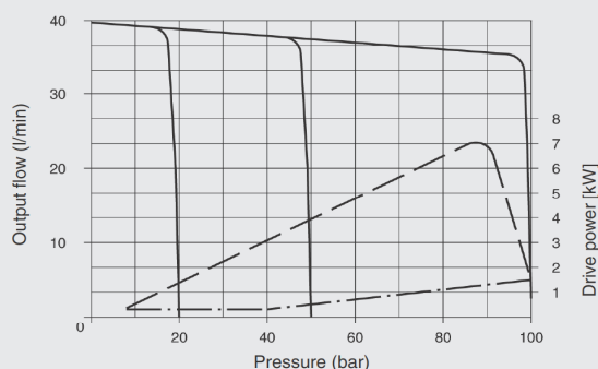
Volumetric efficiency PVV101-1-25
